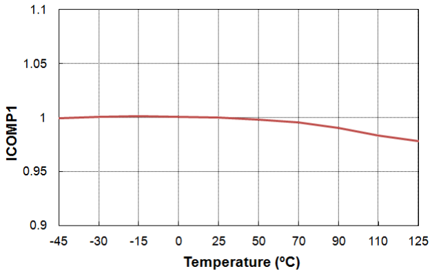
Figure 20. I COMP1 vs. Temperature
