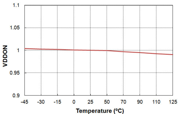
Figure 16. V DD_ON vs. Temperature
