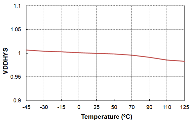
Figure 18. V DD_HYS vs. Temperature
