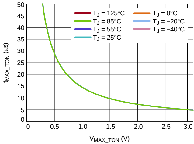
Figure 33. Maximum On-time, ver. Q
