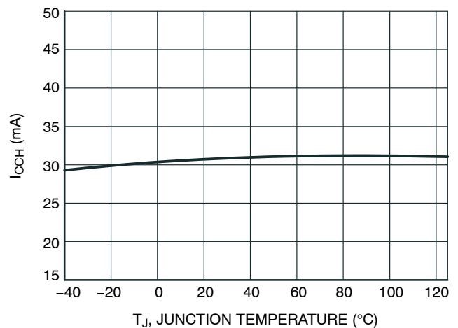
Figure 49. CCH Current to VCCL Pin, V CCH = 8.0 V, V CCCL = 4.0 V
