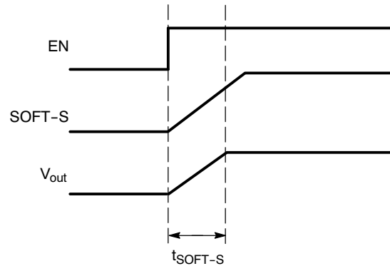
Figure 12. Relationship Between Enable and Soft-Start
