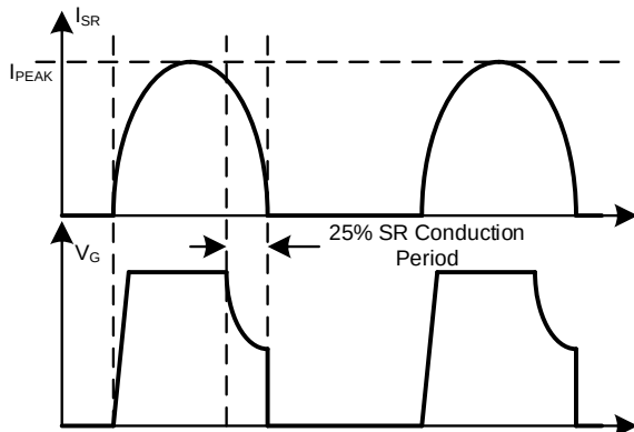
Figure 8: Typical Synchronous Rectification Waveform in LLC
