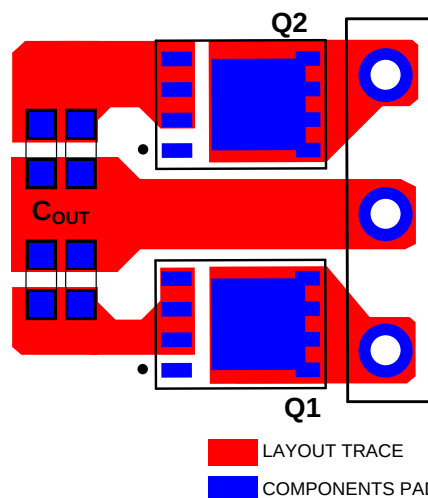
Figure 16: Layout Example for System Power Loop
