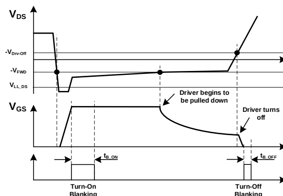
Figure 3: Turn-On/Off Diagram
