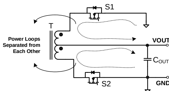
Figure 15: System Power Loop
