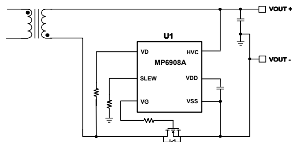
Figure 5: Low-Side Rectification
