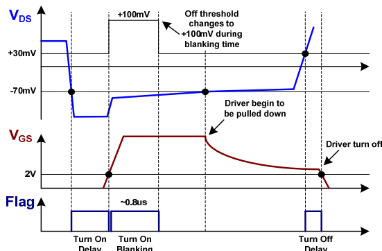
Figure 2: Turn On/Off Timing Diagram
