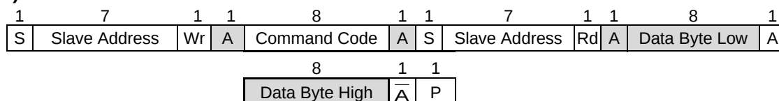
Figure 9: Digital Interface Message Format
