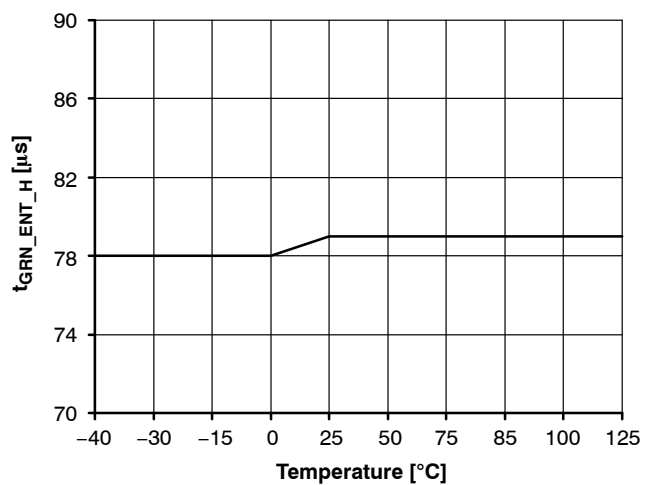
Figure 13. tGRN_ENT_H
