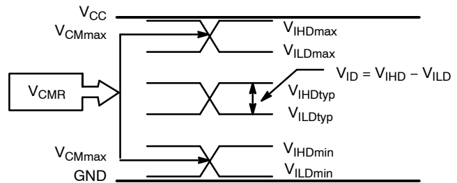
Figure 18. V_{CM} Diagram
