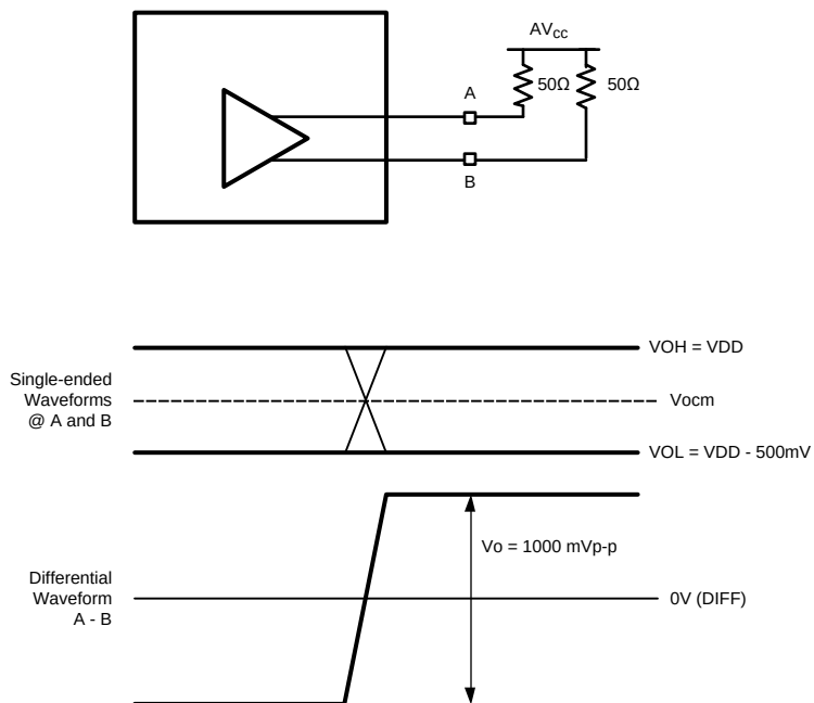
Figure 2. CML Output Swings at A/B ( VOD\_CRL = 24 k\Omega )
