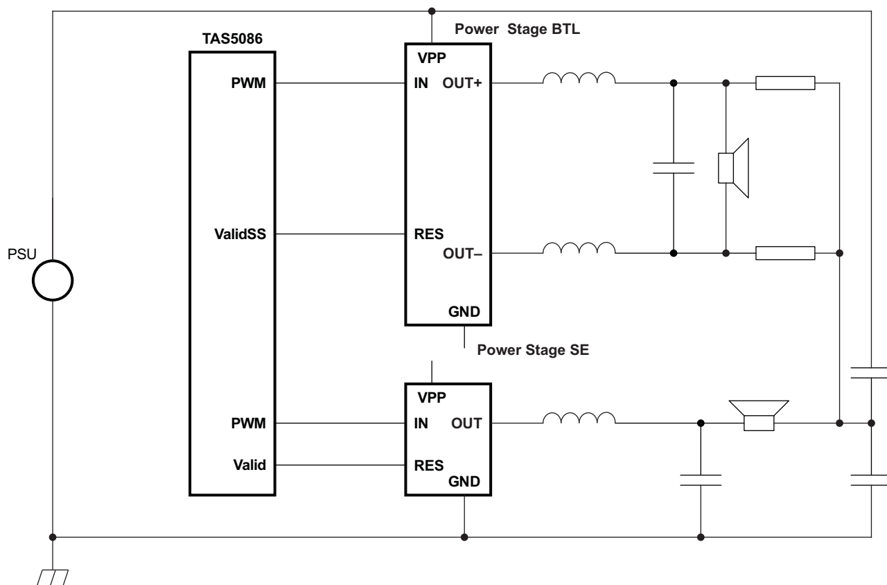
Figure 11. Split-Capacitor Charging With BTL Subwoofer
