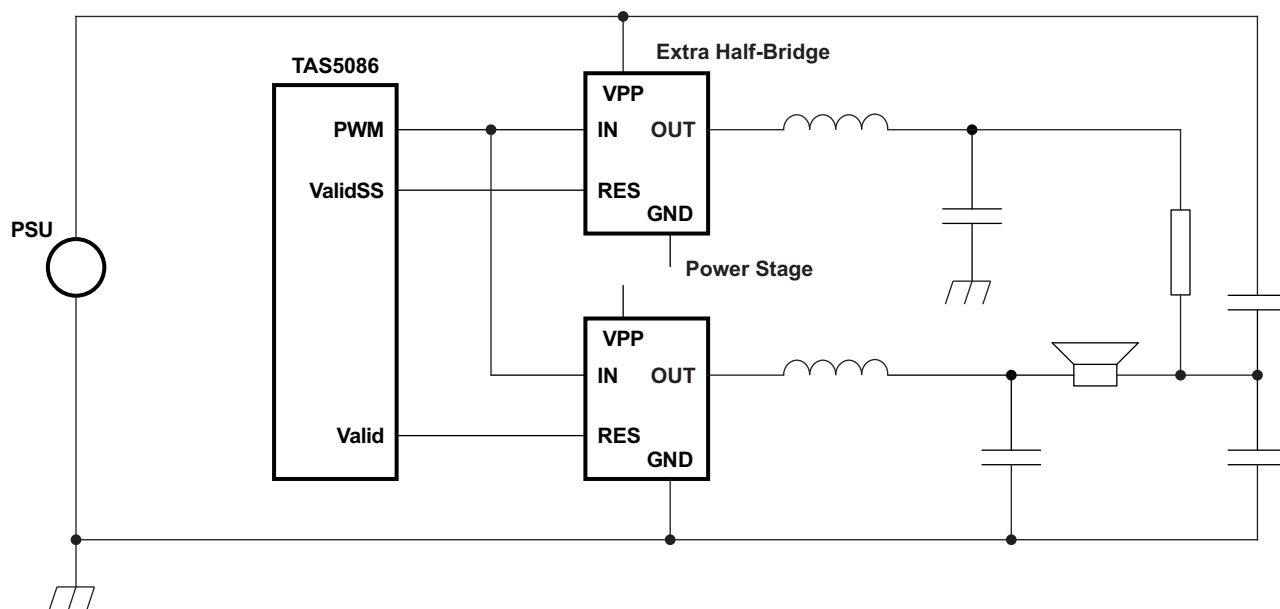
Figure 10. Split-Capacitor Charging With Extra Half-Bridge
