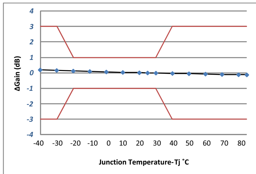
Figure 6. \Delta Gain vs. Temperature (Nominal Temperature = 25°C)
