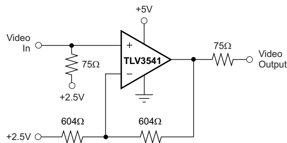
Figure 23. Single-Supply Video Line Driver
