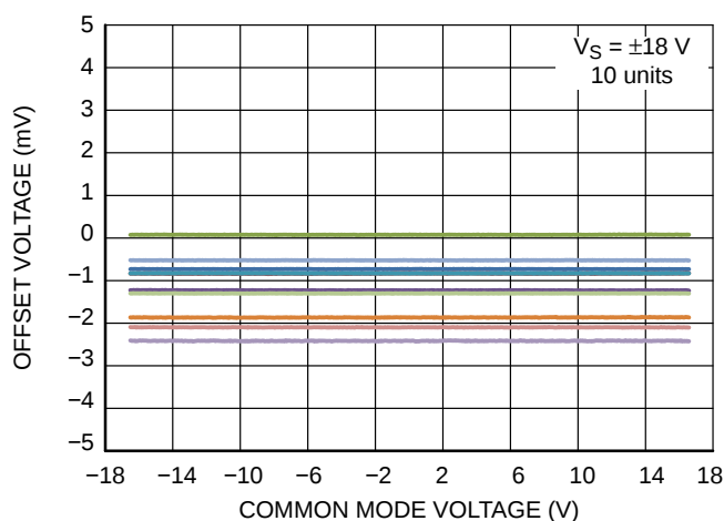
Figure 5. Input Offset Voltage vs. Common Mode Voltage
