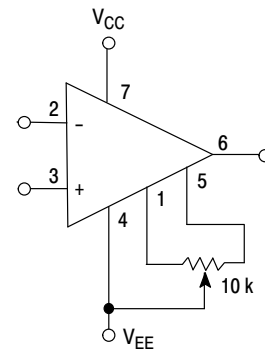
Offset nulling range is approximately \pm 80\text{ mV} with a 10\text{ k} potentiometer (MC33071, MC34071 only).
