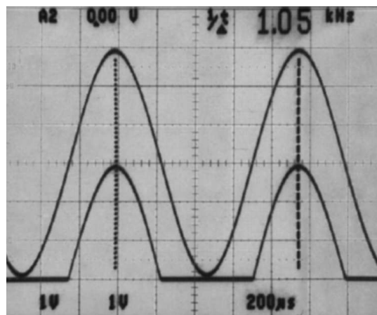
Figure 7-18. Half-Wave Rectifier Waveform
