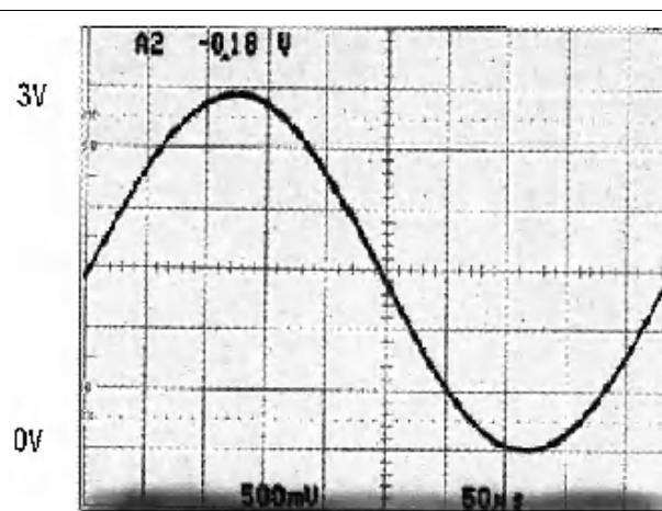
Figure 7-16. Rail-to-Rail Output
