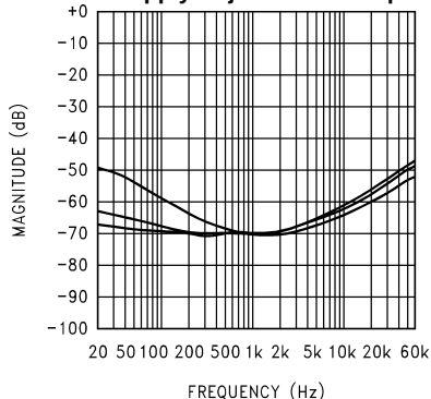
Figure 25. V_{DD} = 12\text{V} , R_L = 8\Omega , BTL operation, V_{\text{RIPPLE}} = 200\text{mV}_{\text{p-p}} , at (from top to bottom at 60Hz): C_{\text{BYPASS}} = 1\mu\text{F} , C_{\text{BYPASS}} = 4.7\mu\text{F} , C_{\text{BYPASS}} = 10\mu\text{F}
