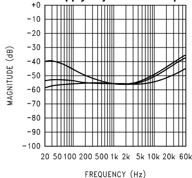
Figure 28. V_{DD} = 12\text{V} , R_L = 8\Omega , SE operation, V_{\text{RIPPLE}} = 200\text{mV}_{\text{p-p}} , A_V = 10 , at (from top to bottom at 60Hz): C_{\text{BYPASS}} = 1\mu\text{F} , C_{\text{BYPASS}} = 4.7\mu\text{F} , C_{\text{BYPASS}} = 10\mu\text{F}
