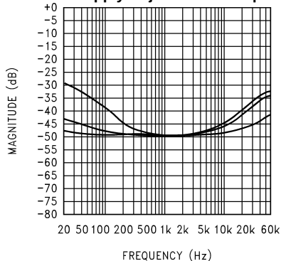
Figure 27. V_{DD} = 12\text{V} , R_L = 8\Omega , BTL operation, V_{\text{RIPPLE}} = 200\text{mV}_{\text{p-p}} , A_V = 20 , at (from top to bottom at 60Hz): C_{\text{BYPASS}} = 1\mu\text{F} , C_{\text{BYPASS}} = 4.7\mu\text{F} , C_{\text{BYPASS}} = 10\mu\text{F}
