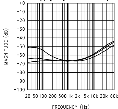
Figure 26. V_{DD} = 12\text{V} , R_L = 8\Omega , SE operation, V_{\text{RIPPLE}} = 200\text{mV}_{\text{p-p}} , at (from top to bottom at 60Hz): C_{\text{BYPASS}} = 1\mu\text{F} , C_{\text{BYPASS}} = 4.7\mu\text{F} , C_{\text{BYPASS}} = 10\mu\text{F}
