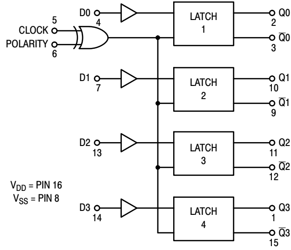
LOGIC DIAGRAM
