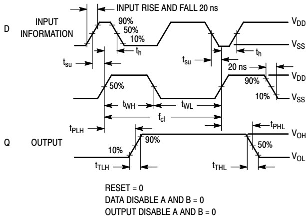
Figure 1. Timing Diagram
